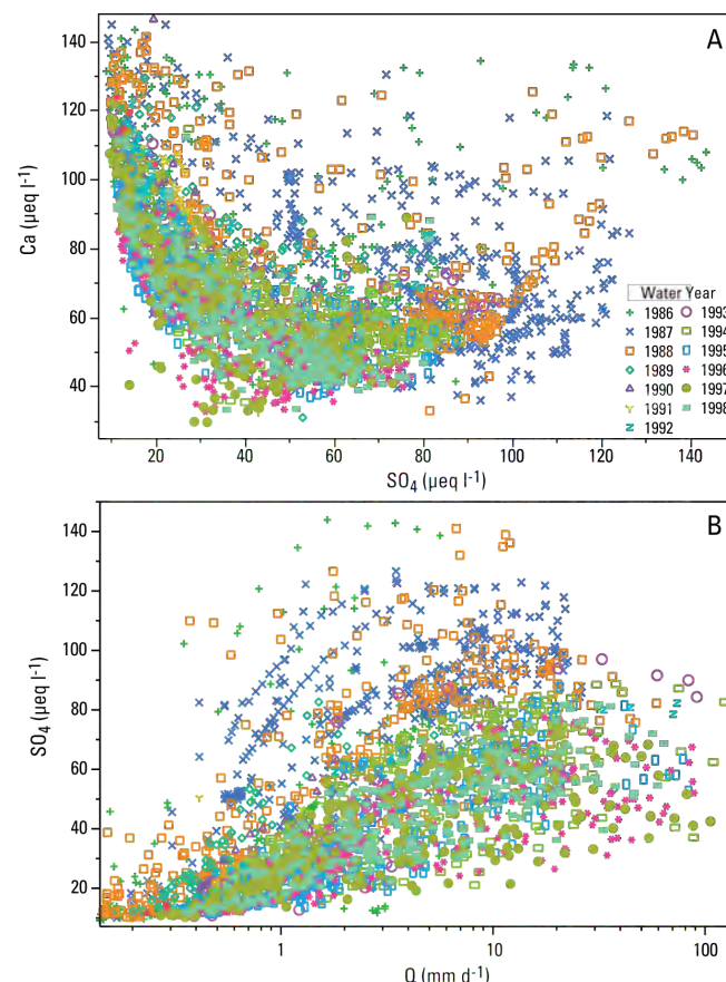
Figure 3. Relations between (A) Ca and \text{SO}_4 concentration, and (B) \text{SO}_4 concentration and runoff subdivided by water during WY1986–1998.
