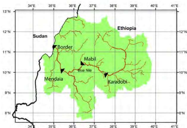
Figure 1. Plan view of proposed hydroelectric dams along the Blue Nile River, as proposed by the United States Bureau of Reclamation.
